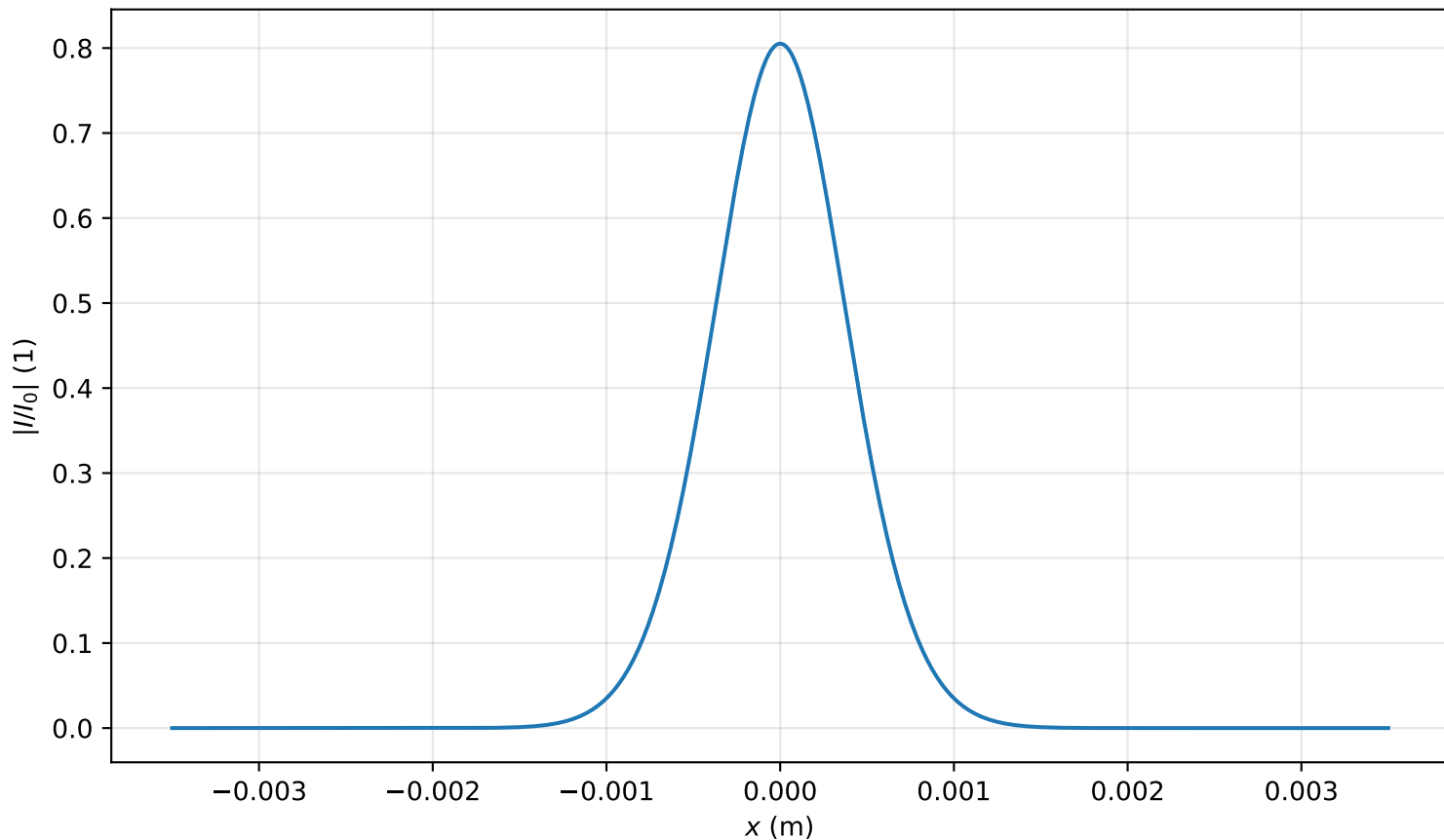
Intensity profile I(x, y = 0, z = 1.274m)/I_0 , P_{in}=0.2P_{cr} , artificial time
